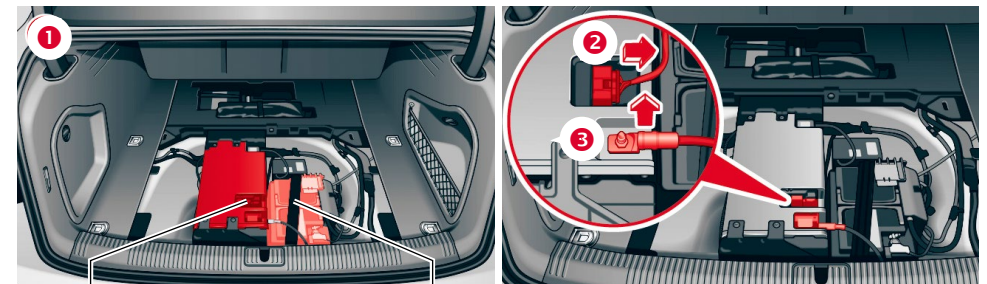
48-volt battery
